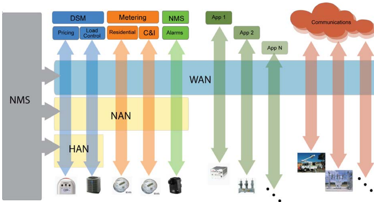
Figure 1 – multiple applications, each partitioned into their own virtual network domain
