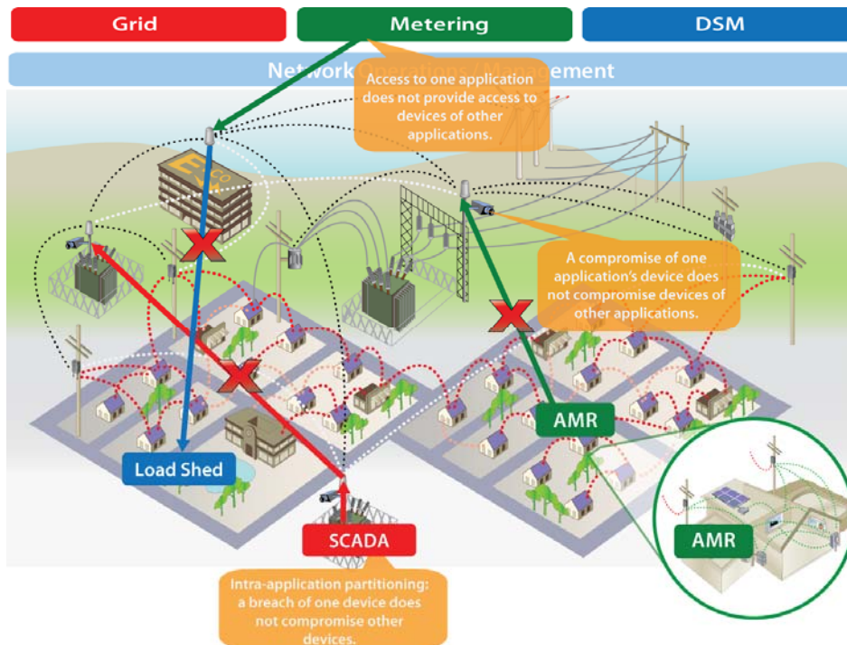
Figure 2 – applications communications secured from breaches
